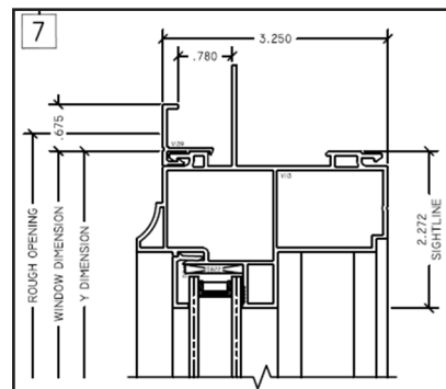
Nail Fin with J-Channel
