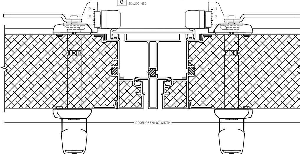
8 REMOVABLE MULLION SD4200 NEG
