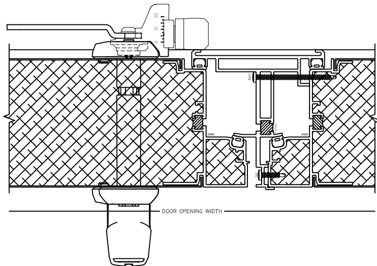
5 APPLIED MULLION SD4200 NEG
