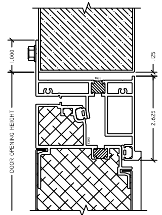
3 HEAD SD3200 NEG
