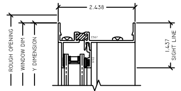
5 HEAD S260 SH
