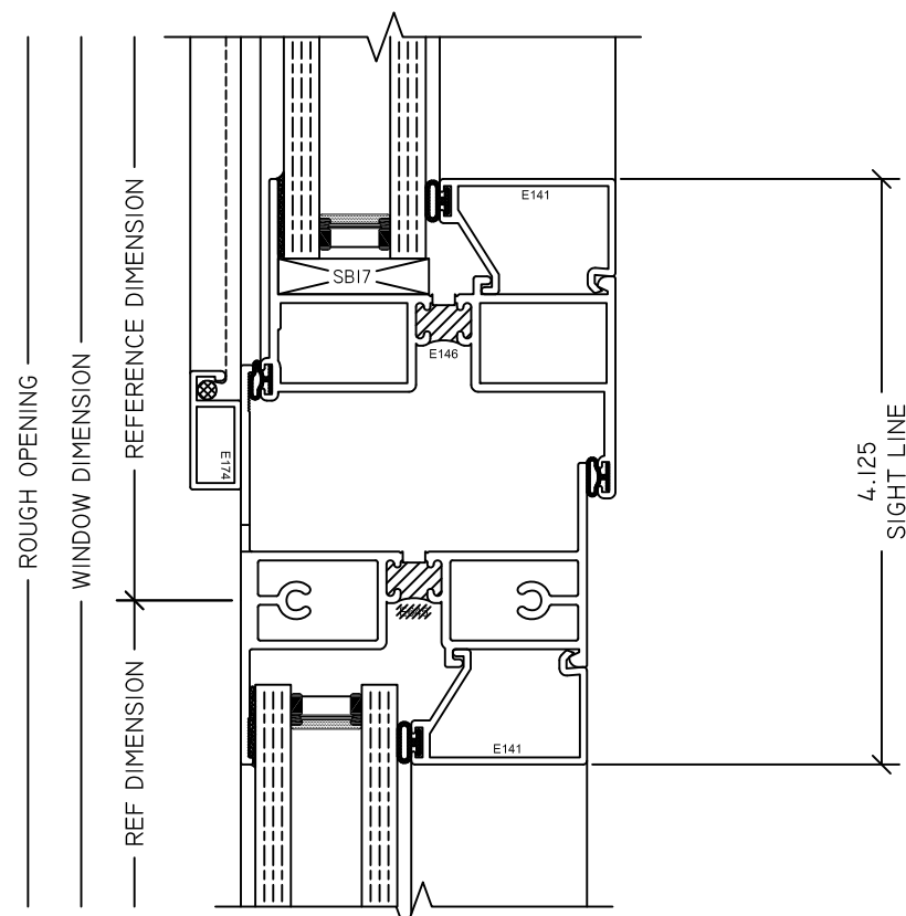
5 PI/FX MTG RAIL S220 PI
