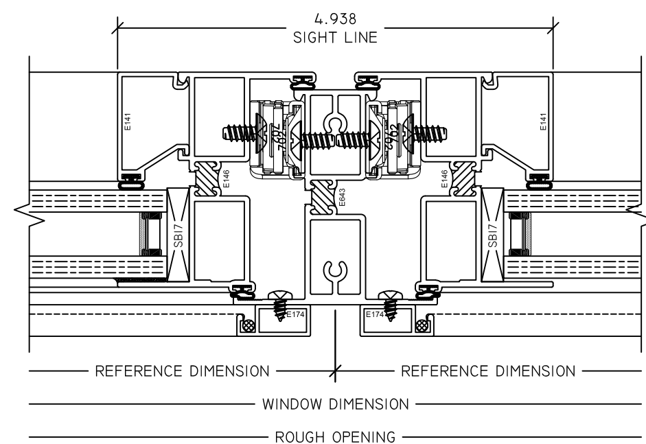
6 PI-PI MTG RAIL S220 PI
