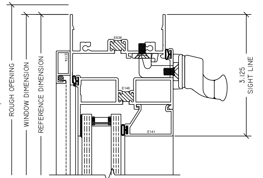
3 PI HEAD S220 PI
