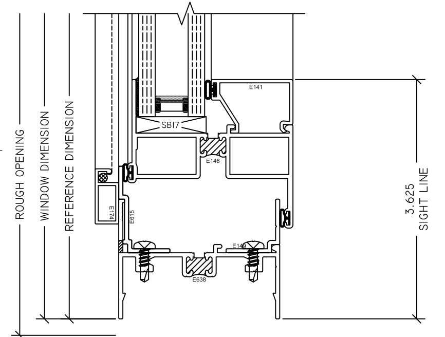
4 PI SILL S220 PI
