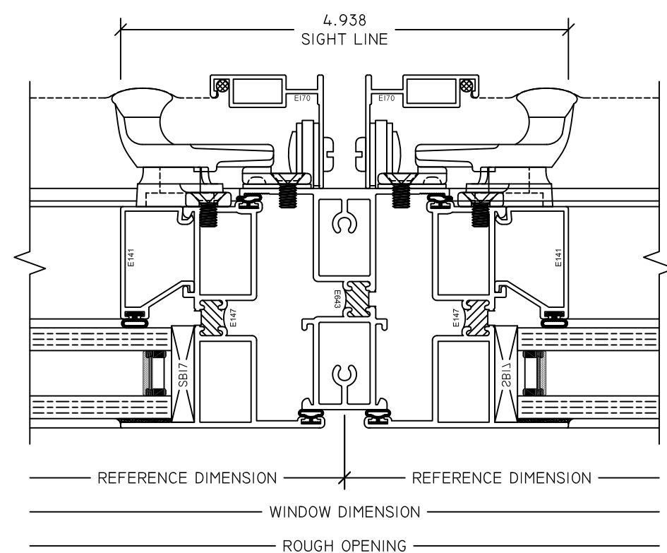
6 CO-CO MTG RAIL S220 OUTSWING
