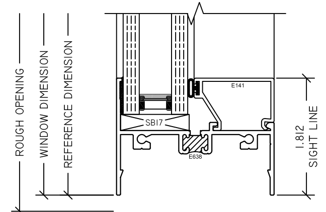
3 FX SILL S220 FXD
