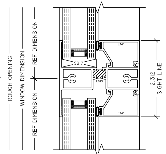
2 FX MUNTIN S220 FXD
