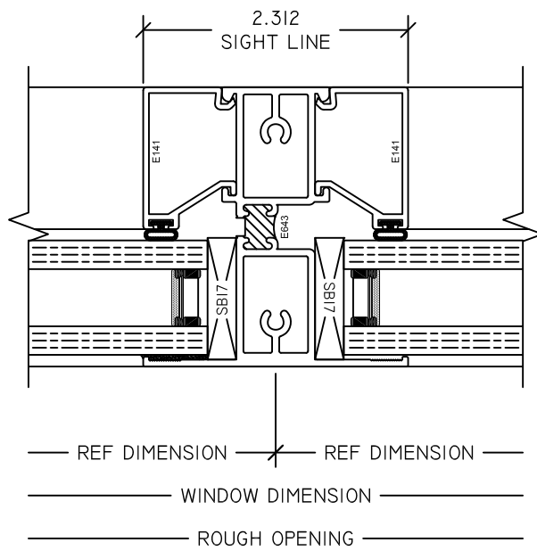
5 FX MUNTIN S220 FXD
