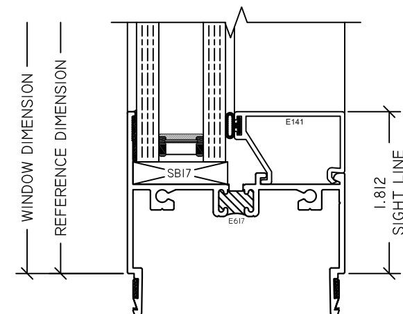
9 STACK SILL S220 FXD
