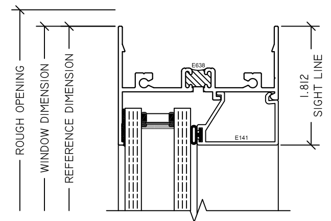
1 FX HEAD S220 FXD
