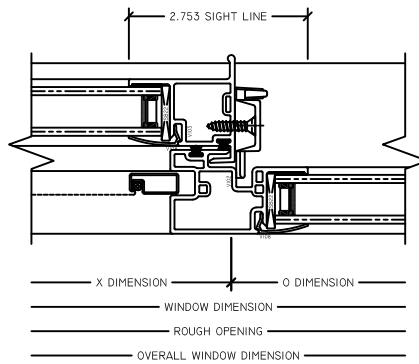
6 XO MTG. RAIL RV STANDARD FIN SLIDER
