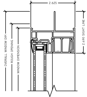
3 FX HEAD RV STANDARD FIN SLIDER
