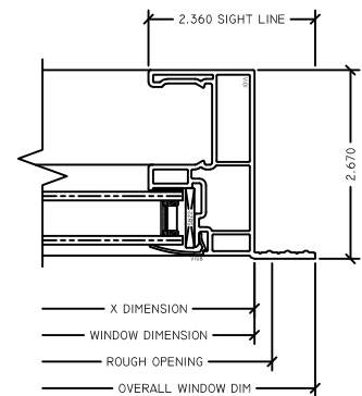
7 FX JAMB RV OUTSIDE FIN SLIDER
