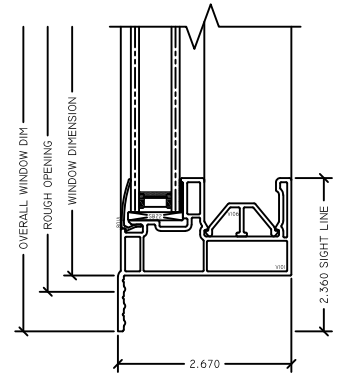
4 FX SILL RV OUTSIDE FIN SLIDER
