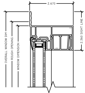
3 FX HEAD RV OUTSIDE FIN SLIDER
