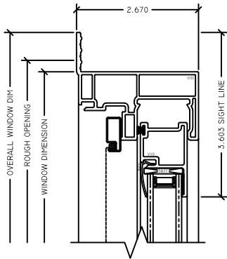
1 OP HEAD RV OUTSIDE FIN SLIDER
