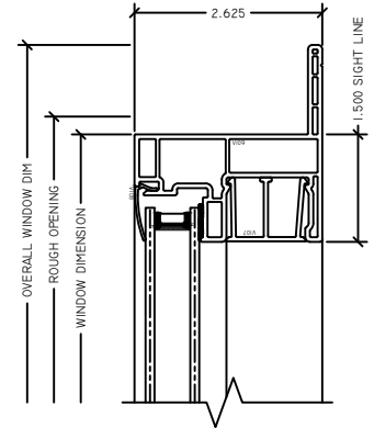
3 FX HEAD RV INSIDE FIN SLIDER
