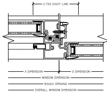
6 XO MTG. RAIL RV INSIDE FIN SLIDER
