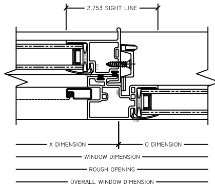
6 XO MTG. RAIL RV INSIDE FIN SLIDER
