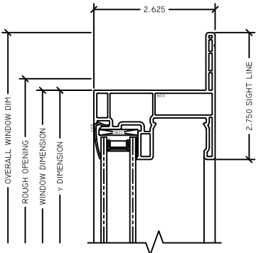
1 HEAD RV INSIDE FIN SH
