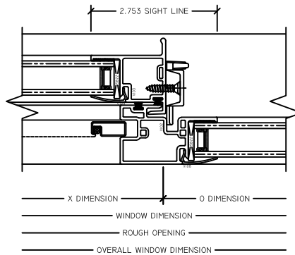
6 XO MTG. RAIL RV BOMAN SLIDER
