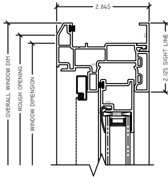
1 OP HEAD RV BOMAN SLIDER
