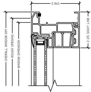
3 FX HEAD RV BOMAN SLIDER
