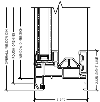
4 FX SILL RV BOMAN SLIDER
