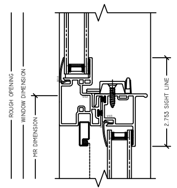
② MTG. RAIL RV BOMAN SH
