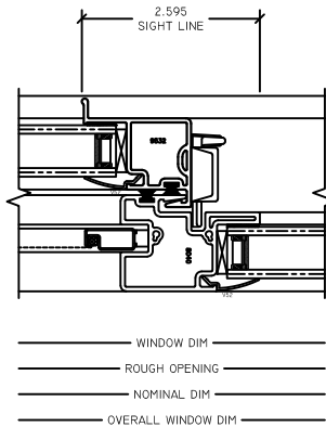
6 MTG RAIL MB70 SLIDER
