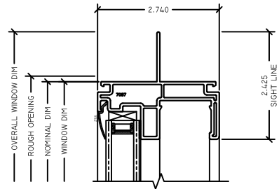
3 FX HEAD MB70 SLIDER
