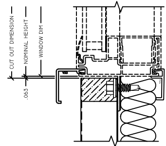
2 FX SILL MB70 TRIM
