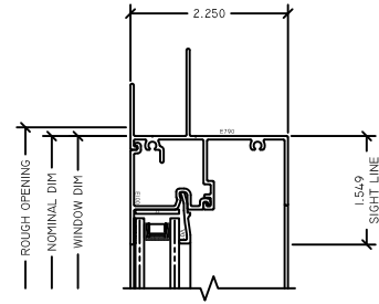
3 FX HEAD M225 SLIDER
