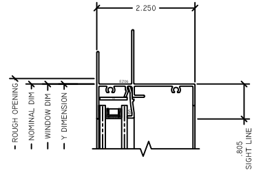
5 HEAD M225 SH
