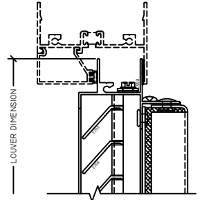
7 HEAD H2211 BLANK OFF
