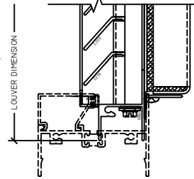
9 SILL H221
