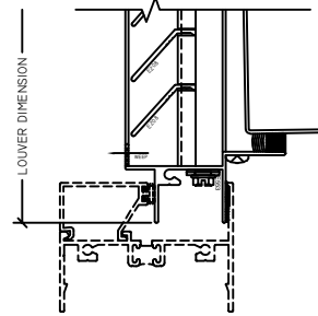
9 SILL H221
