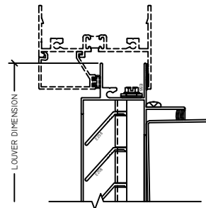
3 HEAD H221
