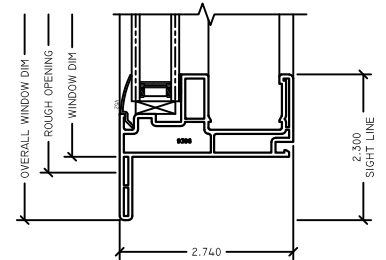
4 FX SILL G75/G78 SLIDER
