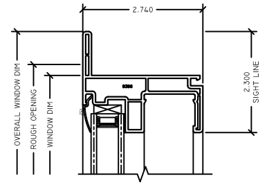
3 FX HEAD G75/G78 SLIDER
