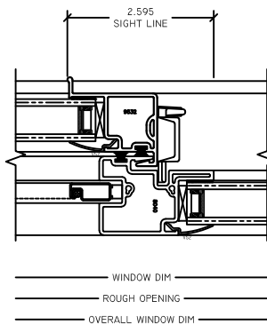
6 MTG RAIL G75/G78 SLIDER
