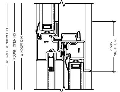
3 MTG RAIL G75/G78 SH
