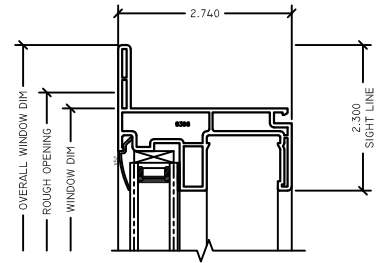
1 FX HEAD G75/G78 SH
