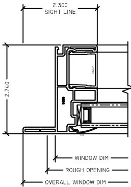
3 FX JAMB G75/G78 FIXED
