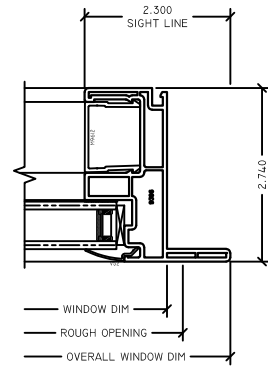
4 FX JAMB G75/G78 FIXED
