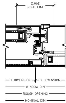
6 MTG RAIL G225 SLIDER
