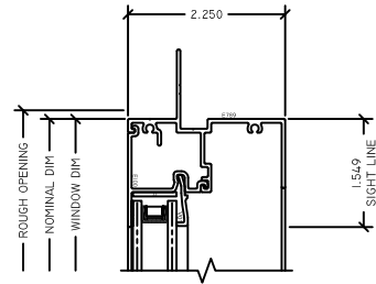
3 FX HEAD G225 SLIDER
