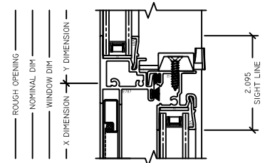
6 MTG RAIL G225 SH
