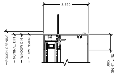
5 HEAD G225 SH
