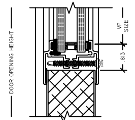
5 VP SILL ADI500 POS
