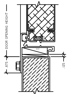
6 SILL ADI500 POS
