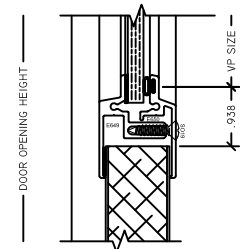
5 VP SILL AD1100 POS
