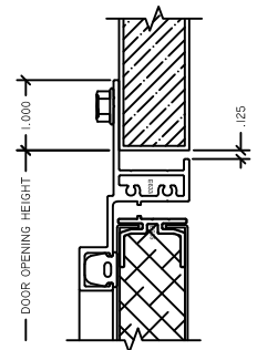
3 HEAD AD1100 POS
