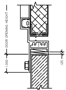
6 SILL AD1100 POS
