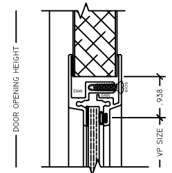
4 VP HEAD AD1100 POS
