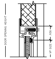
4 VP HEAD AD1100 NEG
