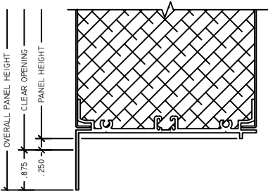
2 PANEL SILL 4" ACCESS PANEL
