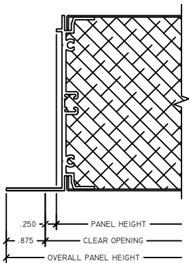
3 PANEL LJAMB 4" ACCESS PANEL
