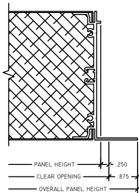
4 PANEL RJAMB 4" ACCESS PANEL
