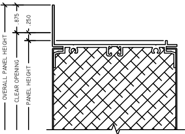
1 PANEL HEAD 4" ACCESS PANEL
