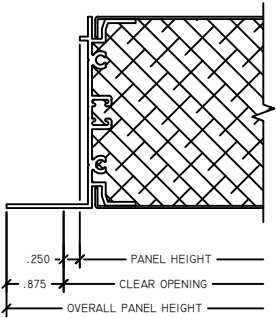
③ PANEL LJAMB 3" ACCESS PANEL
