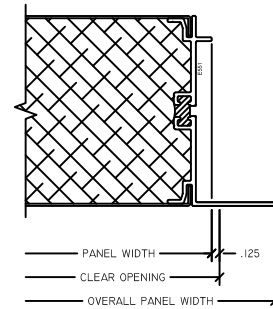
4 PANEL RJAMB 3" ACCESS PANEL
