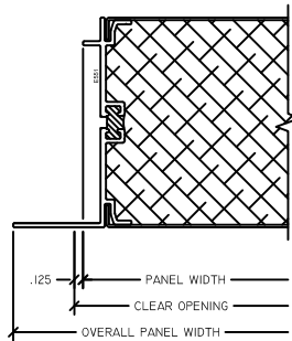
3 PANEL LJAMB 3" ACCESS PANEL
