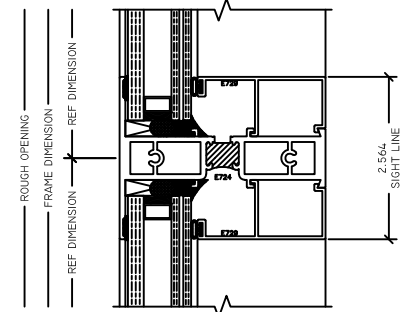
2 HZ FX MTG RAIL 3501 FX
