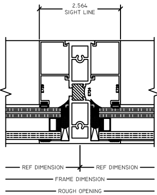
6 VT FX MTG RAIL 3501 FX
