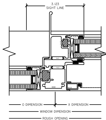
6 OXO MTG RAIL 3210 HS
