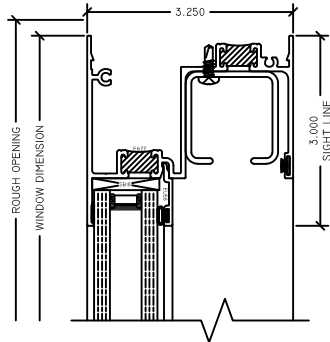
1 FX HEAD 3210 HS
