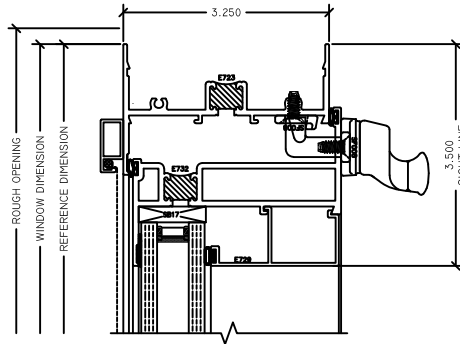
1 PI HEAD 320 PI
