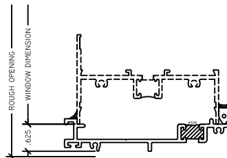
2 SUB SILL
