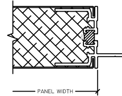
4 PANEL RJAMB 2" ACCESS PANEL
