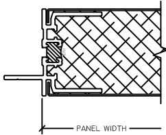
3 PANEL LJAMB 2" ACCESS PANEL
