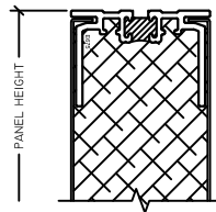
1 PANEL HEAD 2" HVAC PANEL
