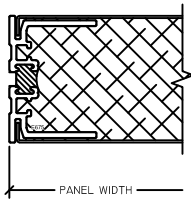
3 PANEL L JAMB 2" HVAC PANEL
