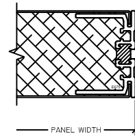
4 PANEL R JAMB 2" HVAC PANEL
