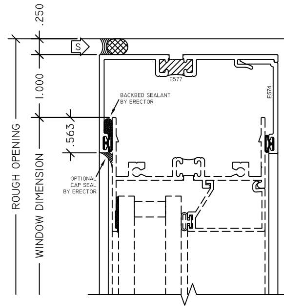
3 HEAD SUBFRAME
