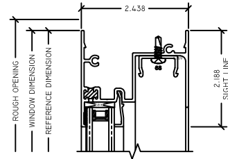
2 FX HEAD 2510 SLIDER
