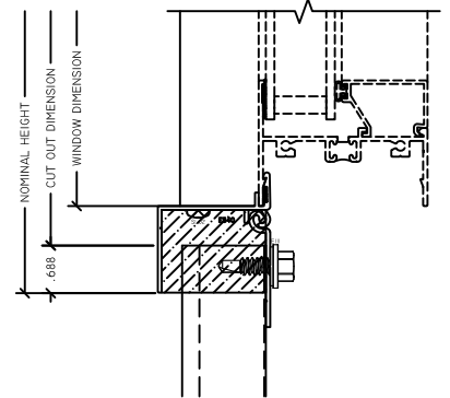
4 SILL ARCHITECTURAL FIN
