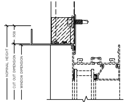
3 HEAD ARCHITECTURAL FIN
