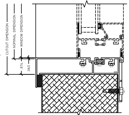
4 SILL 4" INSULVIEW FIN
