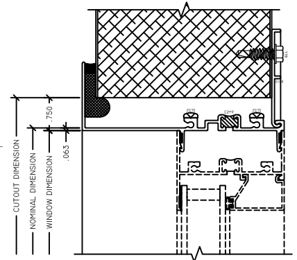
3 HEAD 4" INSULVIEW FIN
