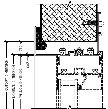
3 HEAD 3" INSULVIEW FIN
