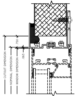
3 HEAD 2" INSULVIEW FIN
