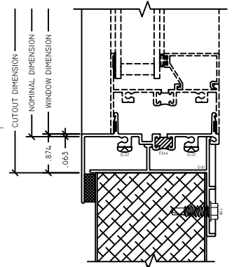
4 SILL 2-1/2" INSULVIEW FIN
