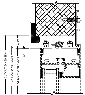
3 HEAD 2-1/2" INSULVIEW FIN
