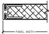
3 PANEL LJAMB 1" HVAC PANEL
