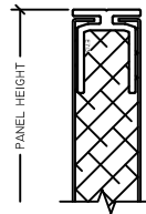
1 PANEL HEAD 1" HVAC PANEL
