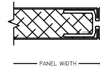
4 PANEL RJAMB 1" HVAC PANEL
