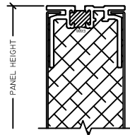
1 PANEL HEAD 1-3/4" HVAC PANEL
