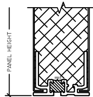
2 PANEL SILL 1-3/4" HVAC PANEL
