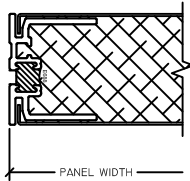
3 PANEL LJAMB 1-3/4" HVAC PANEL
