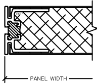
3 PANEL LJAMB 1-1/2" HVAC PANEL
