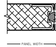
4 PANEL RJAMB 1-1/2" HVAC PANEL
