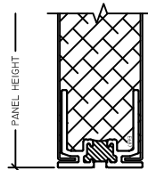
2 PANEL SILL 1-1/2" HVAC PANEL
