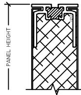
1 PANEL HEAD 1-1/2" HVAC PANEL
