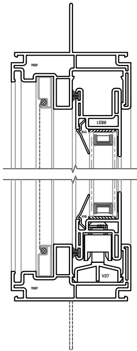
1 SASH HEAD SERIES 70 SLIDER
