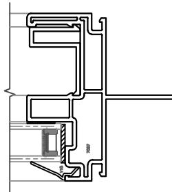
5 FIXED JAMB SERIES 70 HUNG
