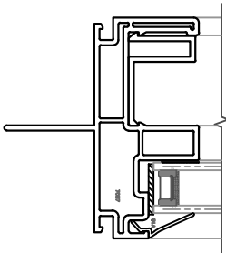
4 FIXED JAMB SERIES 70 HUNG
