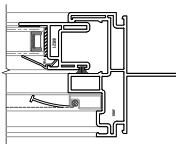
7 SASH JAMB SERIES 70 HUNG
