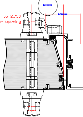
4" DOOR 1 GASKET
