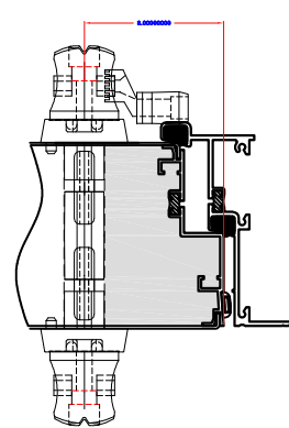
4" DOOR 2 GASKET
